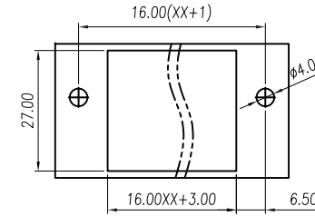
RECOMMENDED MOUNTING CUT-OUT
