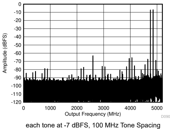
Figure 6-15. DES Mode: Two Tone FFT at 5597 MHz
