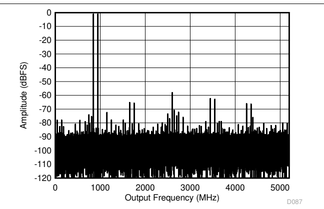
each tone at -7 dBFS, 100 MHz Tone Spacing Figure 6-12. DES Mode: Two Tone FFT at 897 MHz
