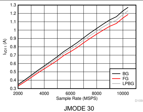
Figure 6-125. DES Mode: I_{VD11} vs Sample Rate
