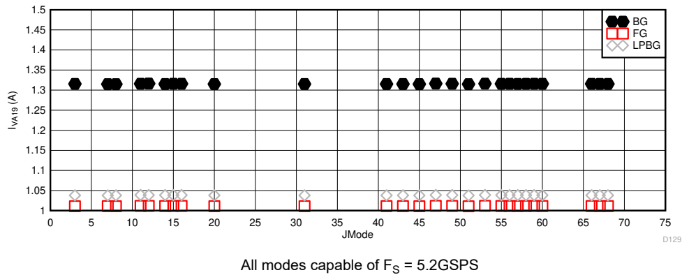
Figure 6-113. Dual Channel Mode: I_{VA19} vs JMODE at 5.2GSPS
