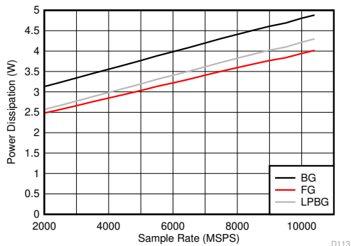
Figure 6-127. DES Mode: Power Dissipation vs Sample Rate
