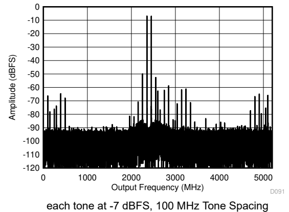
Figure 6-16. DES Mode: Two Tone FFT at 7997 MHz
