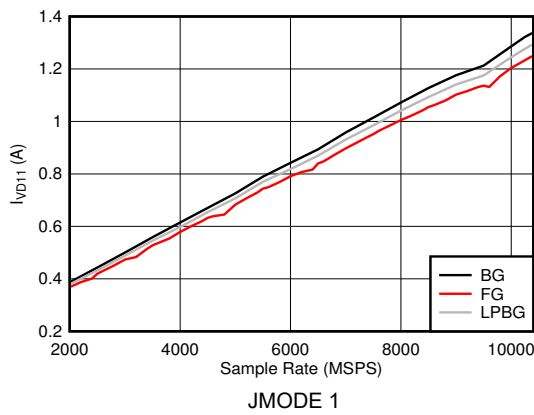
Figure 6-123. DES Mode: I_{VD11} vs Sample Rate
