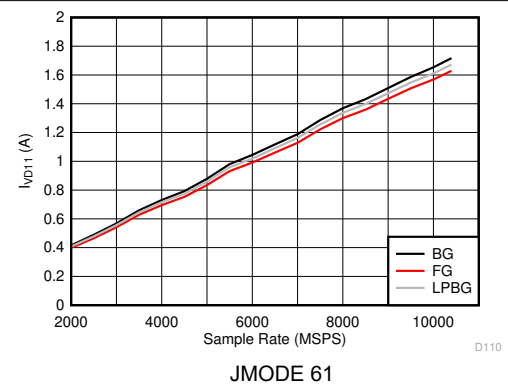
Figure 6-126. DES Mode: I_{VD11} vs Sample Rate
