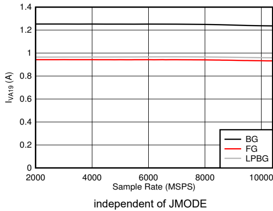
Figure 6-121. DES Mode: I_{VA19} vs Sample Rate
