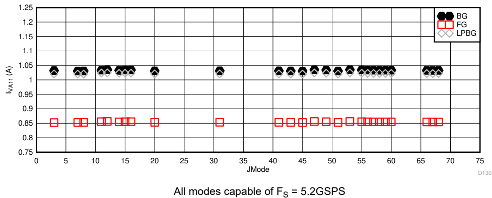
Figure 6-114. Dual Channel Mode: I_{VA11} vs JMODE at 5.2GSPS
