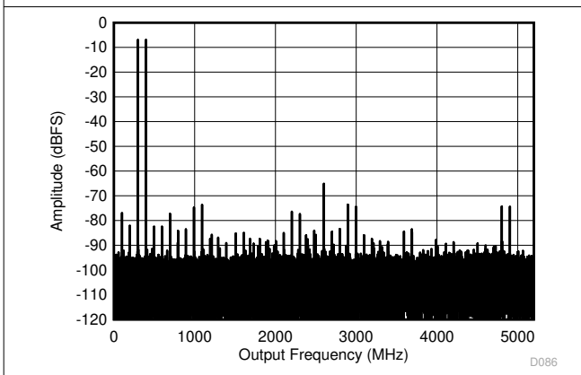
each tone at -7 dBFS, 100MHz Tone Spacing Figure 6-11. DES Mode: Two Tone FFT at 347 MHz
