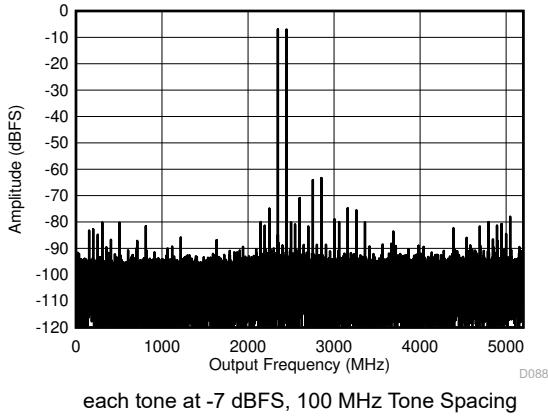
Figure 6-13. DES Mode: Two Tone FFT at 2397 MHz
