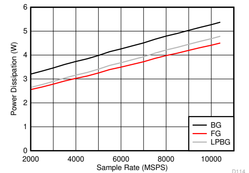
Figure 6-128. DES Mode: Power Dissipation vs Sample Rate
