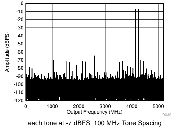
Figure 6-14. DES Mode: Two Tone FFT at 4197 MHz
