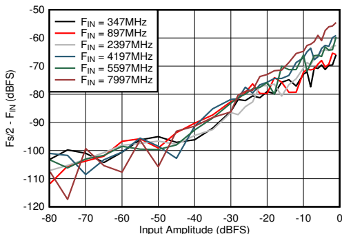
Figure 6-65. DES Mode: F_s/2 - F_{\text{IN}} vs Input Amplitude and Frequency
