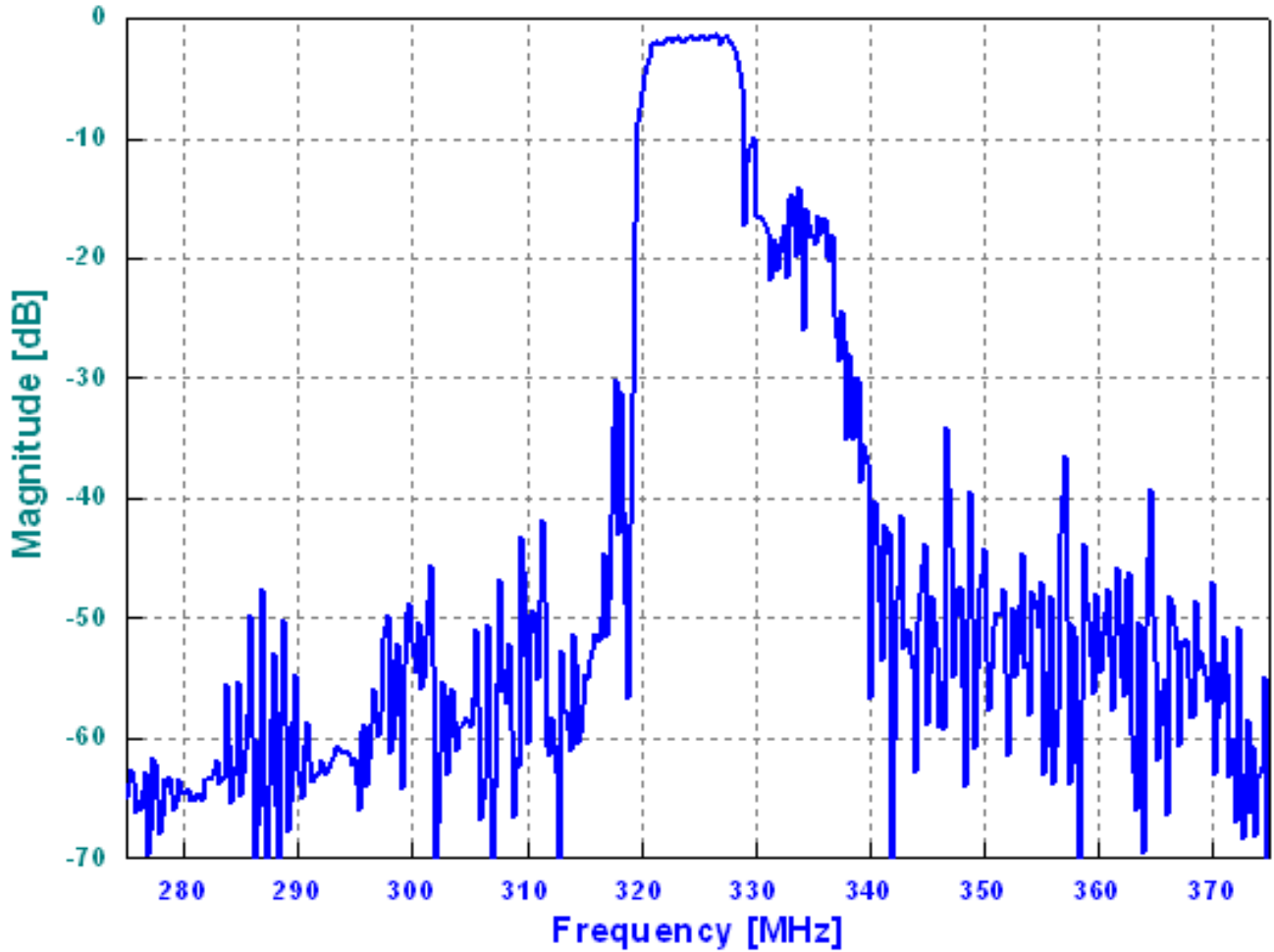
Response Plot:
